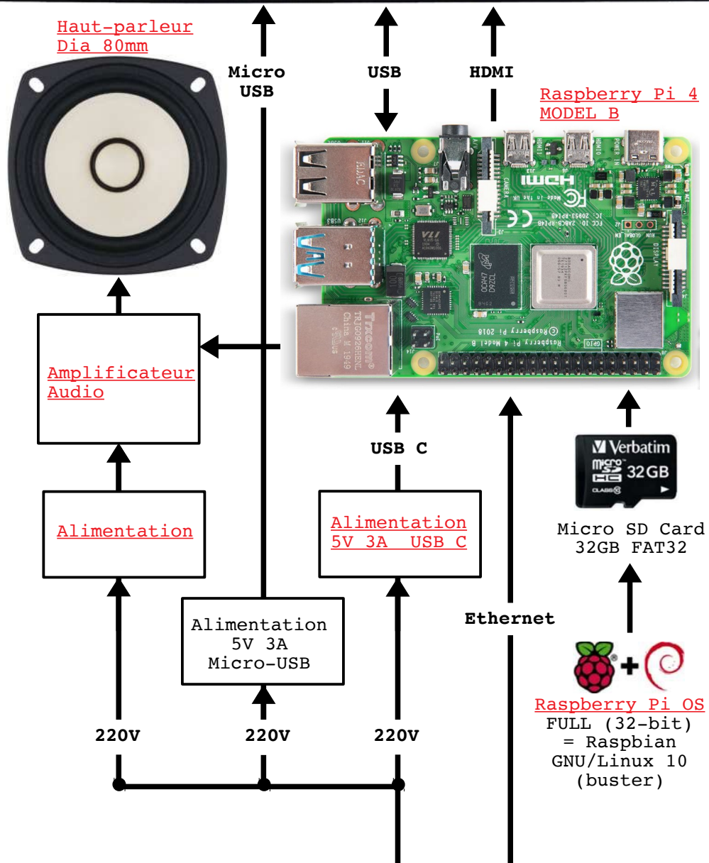
Schema-Raspberry6
